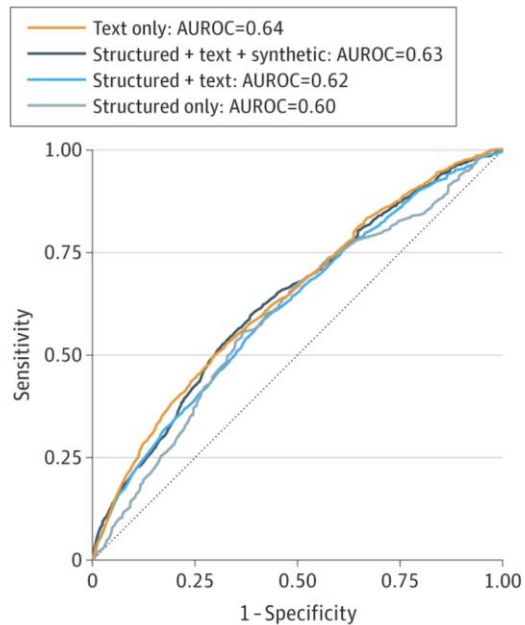
A ROC curve of the best performing models for each feature set on the test set
